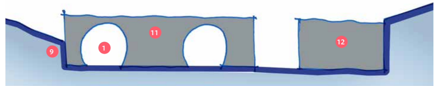
Portal elevation
